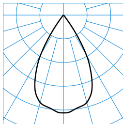
Qui130 G3 RF-VFL-c 50-827 M32 ETBLE 01 TX828595
