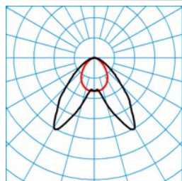
ELINE LDAW55-140 ML 865 L225 0 50 ■ C0 - C180
