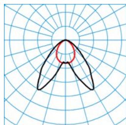
ELINE LDAW55-140 ML 865 L225 2 50
