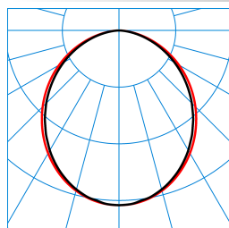
Fn5 3P10 DIL 25-830 ETDD 05 TX562361
