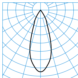
Qui155 G3 RF-FL 20-8ACT M23 ETBLE 01 (ACTDSU) TX828100
