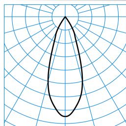
Qui155 G3 RF-FL 20-8ACT M23 ETBLE 01 (ACTDWW) TX828103
