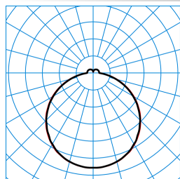
Olisq QWD2 DW 35-830 ETBLE +CAS IP54 TX842404
