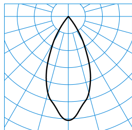
E-Line PRO 78 BV G2 RF-WFL 30-BC M49 ETBLE 05 Blank TX714977
