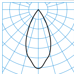
E-Line PRO 78 BV G2 RF-WFL 30-BC M49 ETBLE 05 05 TX716555
