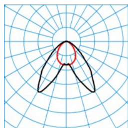
7850 LDAW40-110 ML 865 L150 10 50 ■ C0 - C180
