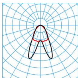
7850 HE LDAN60-160 ML 830 L225 10 50 ■ C0 - C180
