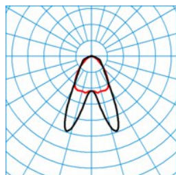
7850 HE LDAN60-160 ML 830 L225 12 50 ■ C0 - C180
