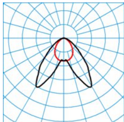
7850 HE LDAH60-160 ML 830 L225 12 50 ■ CO - C180
