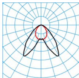
7850 HE LDAW60-160 ML 830 L225 14 50 ■ C0 - C180
