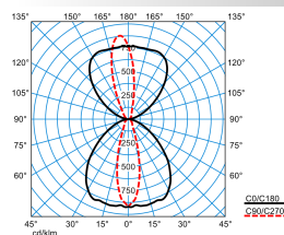
OsidoRW-SB1L/SB1L-20-830-ET-GS26
