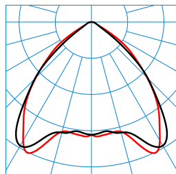
E-Line TB LED8000-865 IP54 TX053452
