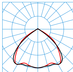
E-Line M-B LED5500-865 IP54 TX053270
