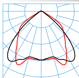
E-Line Act TB LED10000 (ActDWW) TX064337
