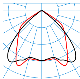
E-Line Act TB LED10000 (ActDCW) TX064335
