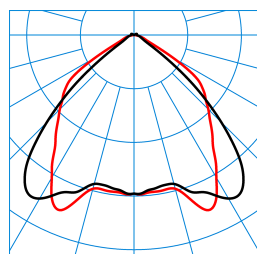
E-Line Act TB LED10000 (ActDSU) TX064336
