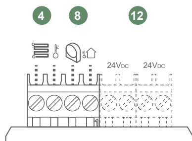
fig. 41 - Raccordements Sondes
