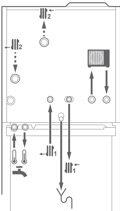
fig. 4 - Raccordements hydrauliques
