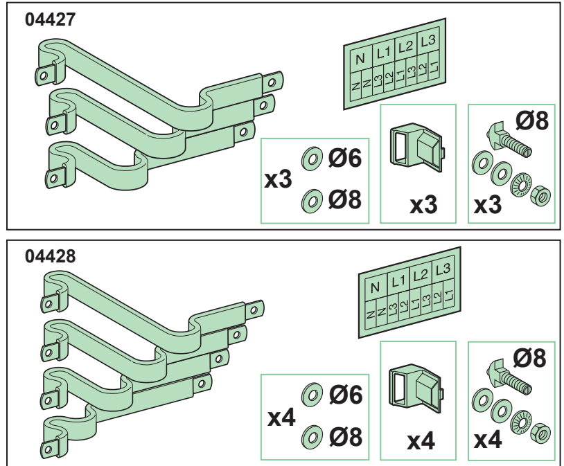
Compact NSX100/160/250 3P/4P Vigi NSX100/160/250 3P/4P INS-INV250 3P/4P
