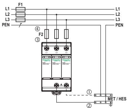
TN-C System, 3+0
