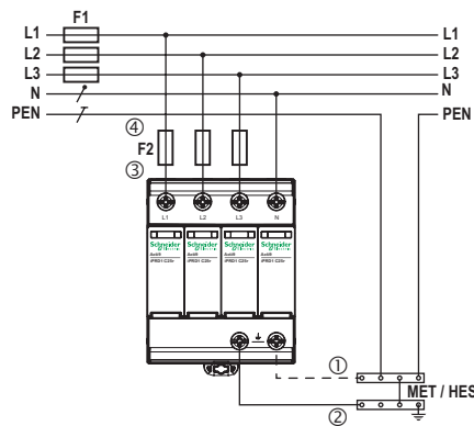
TN-S System, 3+1
