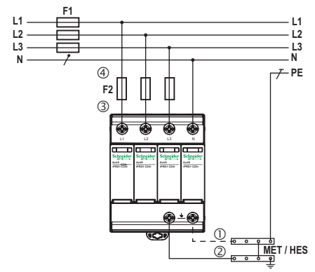
TT System, 3+1
