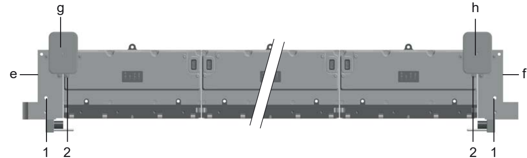
1 Two screws: M6x120 class 8.8 ISO 4762, torque 10.1 Nm (89.4 lbf-in) 2 Four screws: M3x8 ISO 14583, torque 0.6 Nm (5.31 lbf-in)
