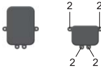
2 Screw: M3x8 ISO 14583, torque 0.6 Nm (5.31 lbf-in)
