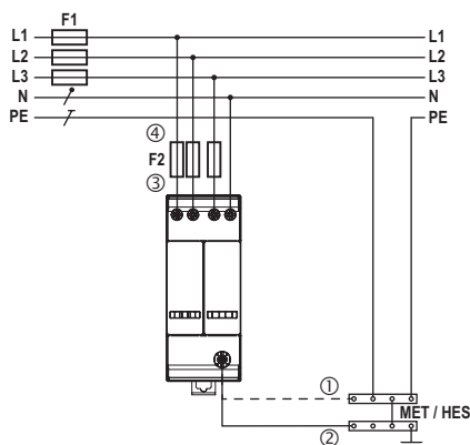
TN-S Network Connection (3+1) A9L2C620
