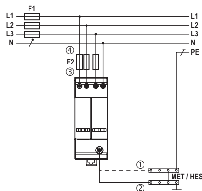
TT Network Connection (3+1) A9L2C620
