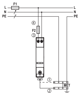
TN-S Network Connection (3+1) A9L2C620
