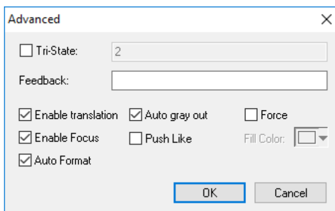
Advanced dialog
