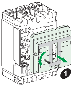
NSX100-250 + MicroLogic 2.2
