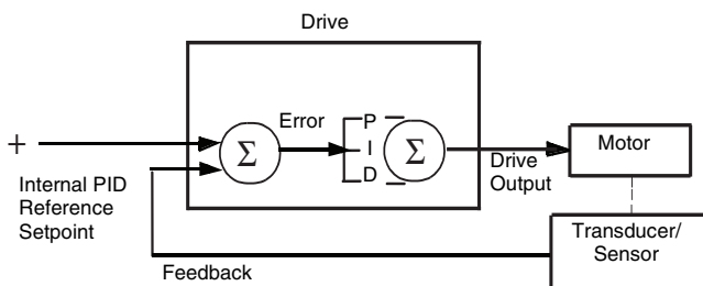
Figure 5 – PID Setup for Drive
