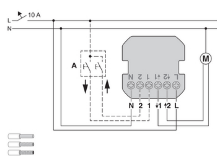
(A) Mechanical push-button (optional)
