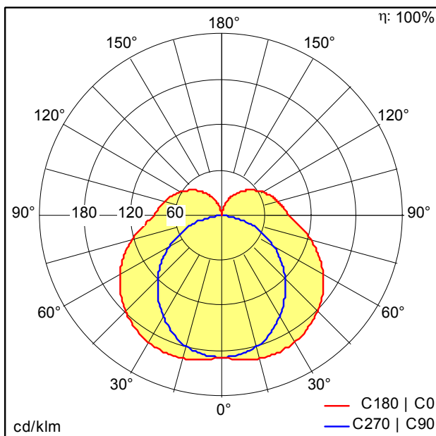
D39718AA_LINARIA_LED1500-840_L608_PM_SR.Idt
