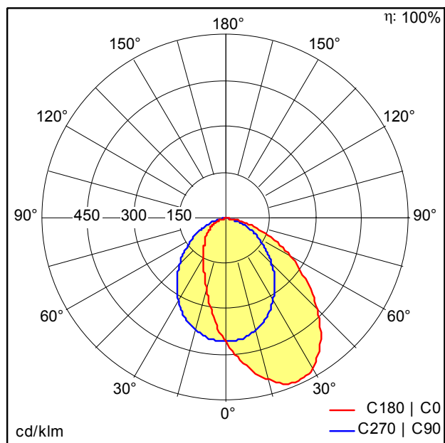
D42966AA_SLOIN_LED2600-840_L1000_WW_HO.Idt
