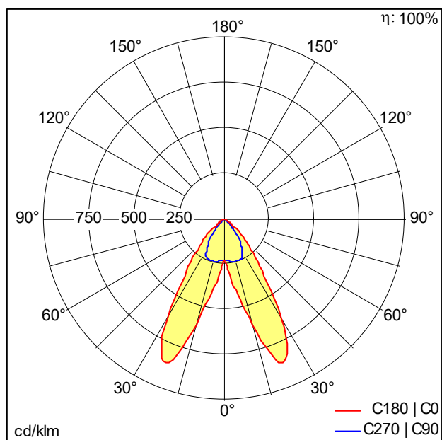
Sceno_(2x7)_3500-830_DA_re.Idt, Sceno_(2x7)_3500-830_DA_li.Idt
