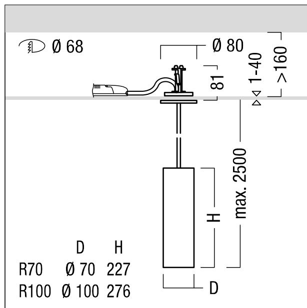
ZS_PA_I_M_R_PEND_R_LDO.wmf
