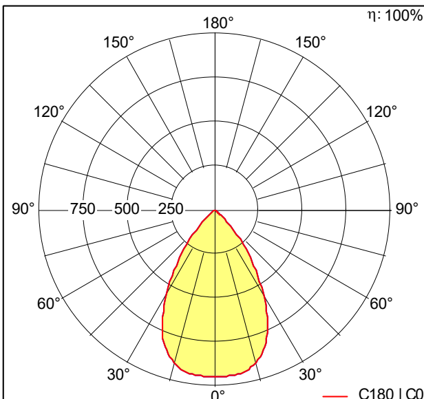
PANOS_R_R_100_2k-830_SWI_L_AL_WH.Idt
