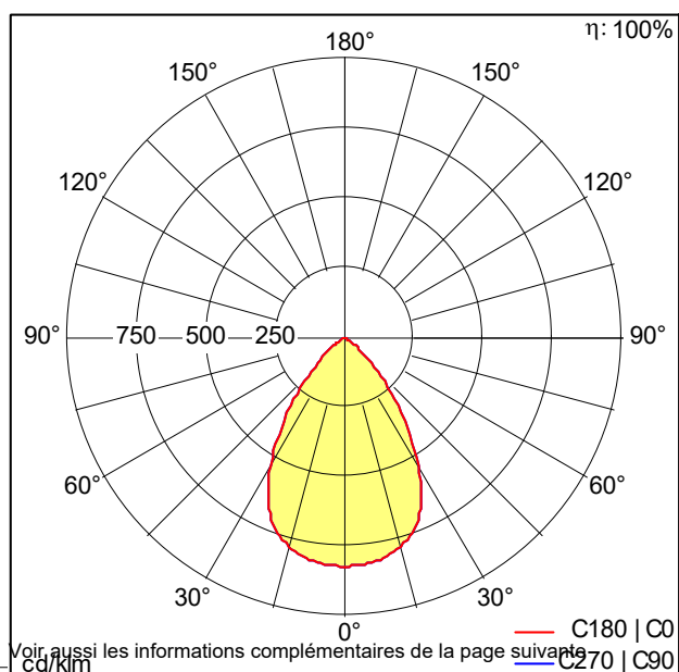
PANOS_R_R_100_1k-940_SWI_L_SPC_WH.Idt
