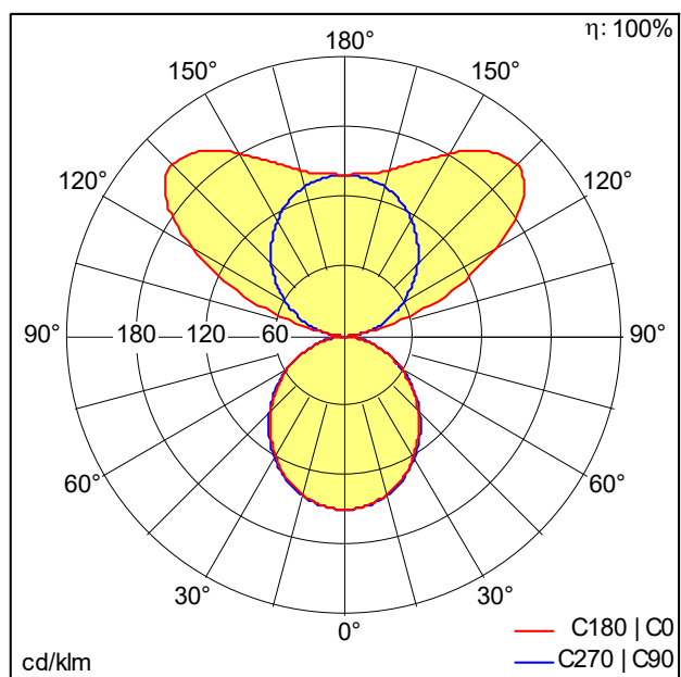
D42843AA_D44967AA_SLOIN_SLIM_ID_840_L1250_PC_WH.Idt
