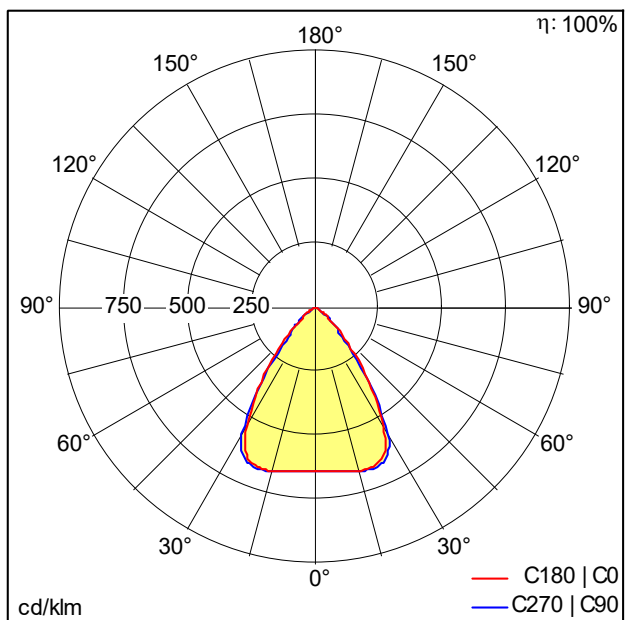
D49207_SLN2-B_2500-Z40_L2000_MC_LDE_BKM.Idt
