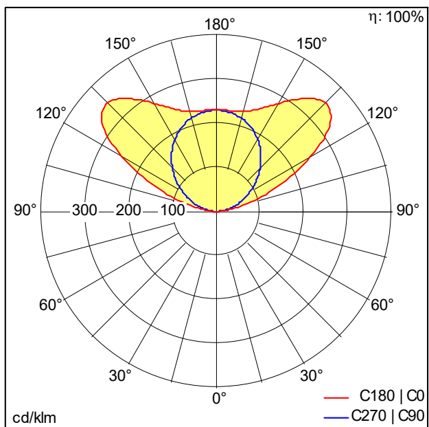
D46423_SLN2-C_1600-Z40_L1500_WH.Idt
