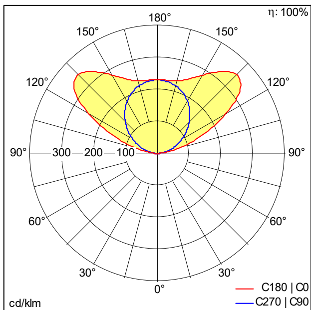
D46423_SLN2-C_1600-Z40_L3250_WH.Idt
