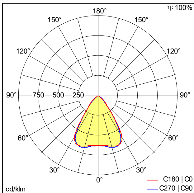
D50394_SLN2-B_L1750_3500_BKG_WW.Idt
