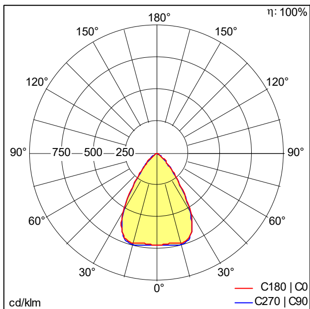
D50390_SLN2-B_L1750_3500_SRG_WW.Idt
