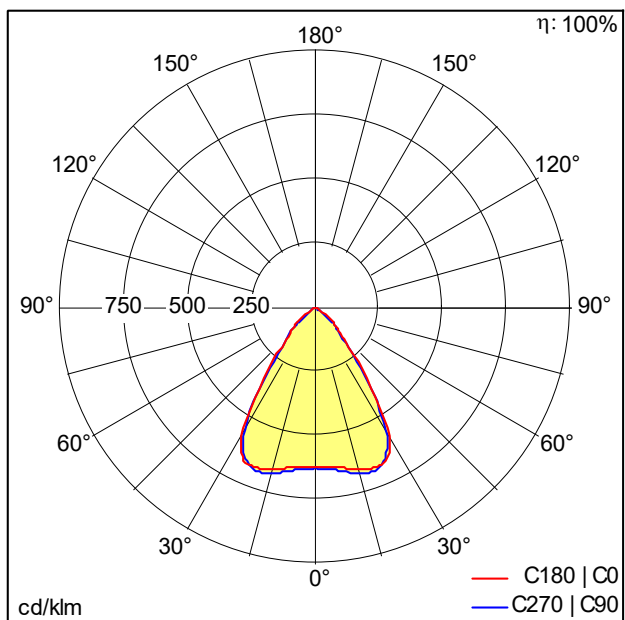
D50394_SLN2-B_L2000_3500_BKG_WW.Idt
