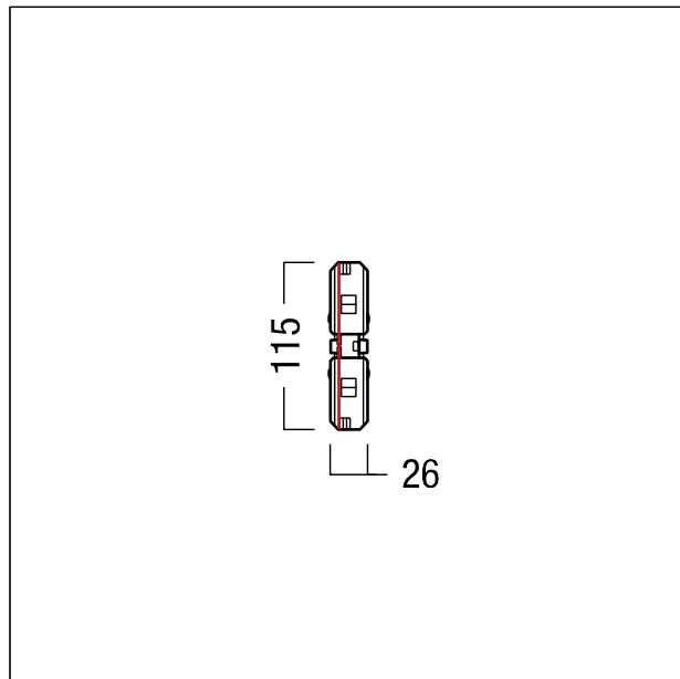
ZS_ZTB_M_3PH_DALI_ELEC_CON.wmf
