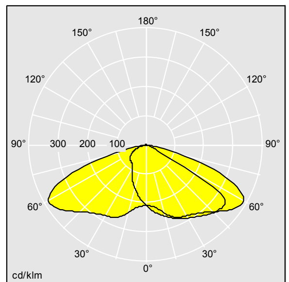
TL_THLOD48L50SC740.ltd
