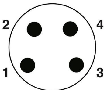
Pin assignment M8-plug, 4-pol, A-coding
