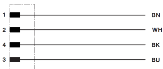
Pin assignment M12-plug
