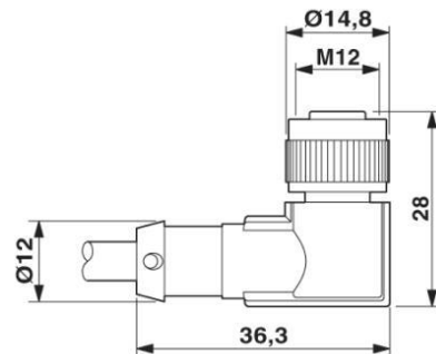
Jack M12 x 1, angled
