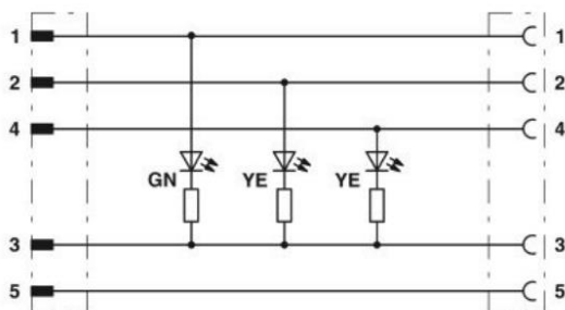
Pin assignment between M12-plug and M12-jack with LED
