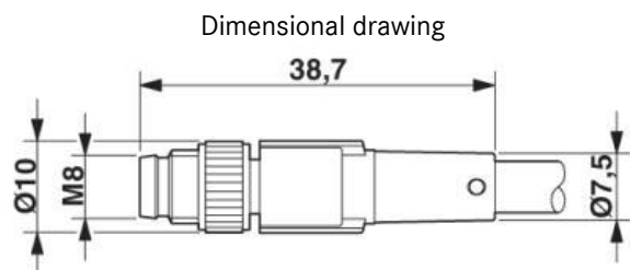
Plug M8 x 1, straight
