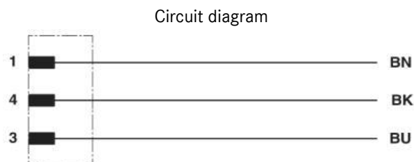
Pin assignment from M8-plug
