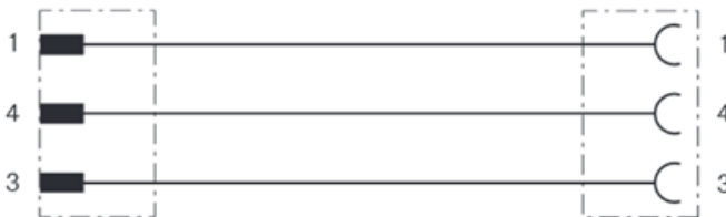
Pin assignment between M8-plug and M12-jack
