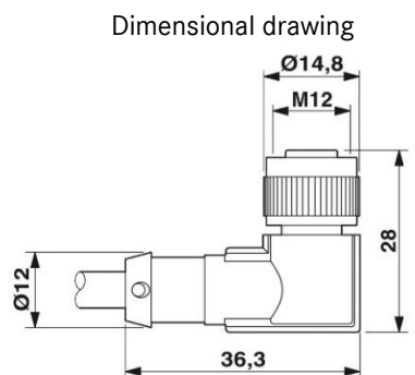
Jack M12 x 1, angled, with LED
