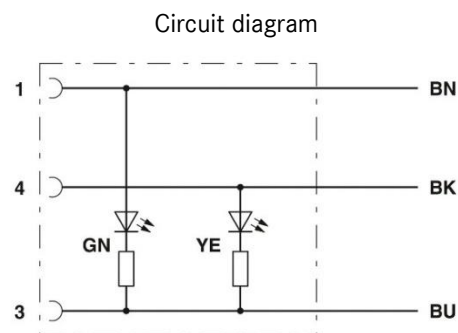
Pin assignment M12-jack
