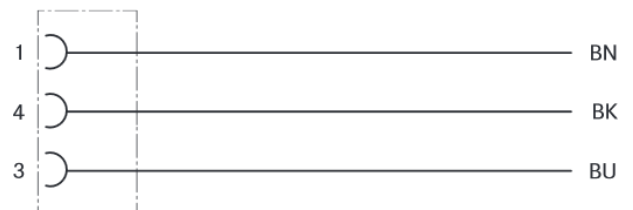
Pin assignment M12-jack
