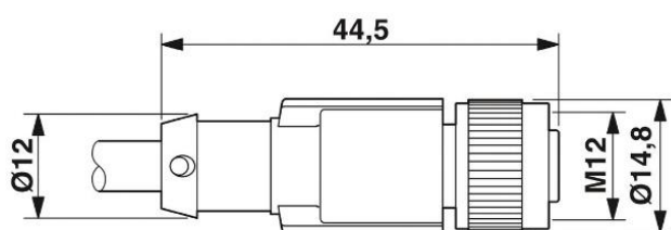
Jack M12 x 1, straight, with LED
