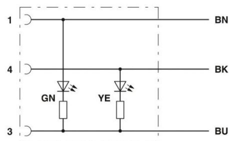
Pin assignment M12-jack
