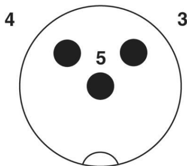
Pin assignment
