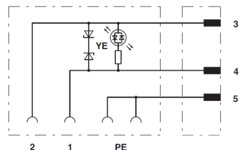
Pin assignment between M12-plug and valve connector
