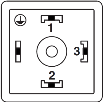
Valve connector, type AD
