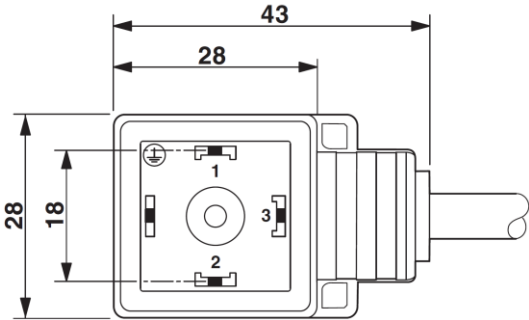
Valve connector, type AD
