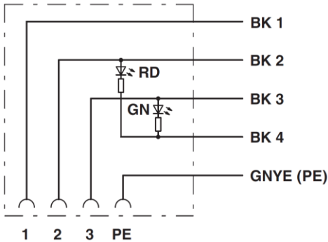
Pin assignment of valve connector
