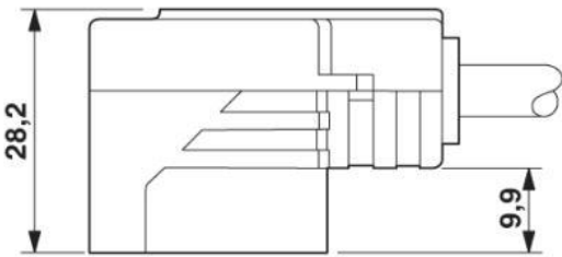
Valve connector, type AD, side view
