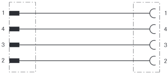
Circuit diagram
