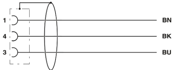
Pin assignment from M12-jack
